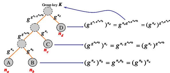
Figure 17: Illustration of STR
