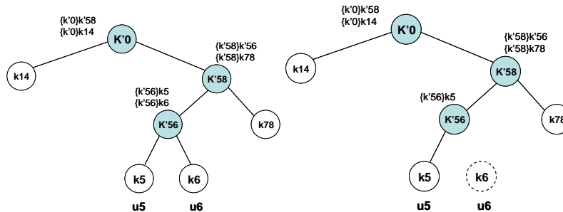
Figure 11: Illustration of joining member U_5
