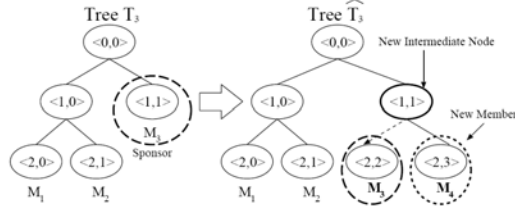
Figure 15: Illustration of join member in TGDH
